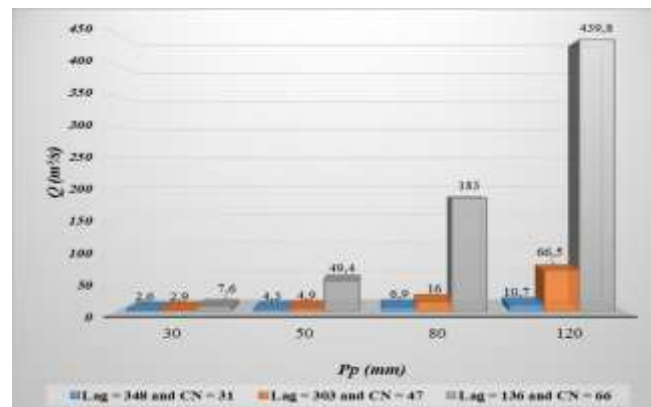
Fig. 8 Simulated flows in conditions of afforestation degree of 80% for different amounts rainfall fallen in 1hour
