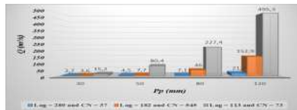
Fig. 13 Simulated flows in conditions of deforestation degree of 15% for different amounts rainfall fallen in 6 hour
