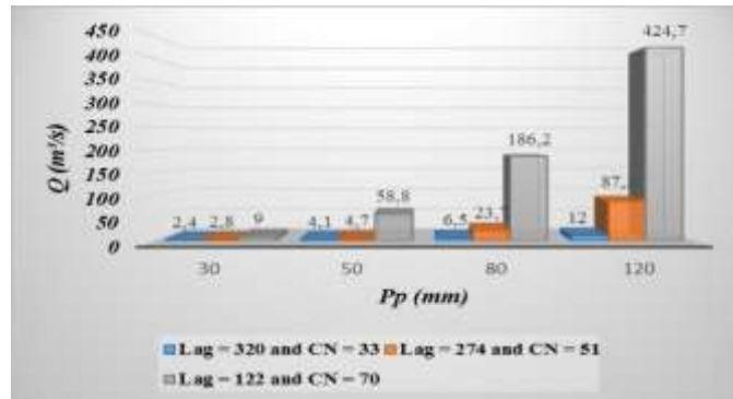
Fig. 7 Simulated flows in current conditions of afforestation for different amounts rainfall fallen in 6hour
