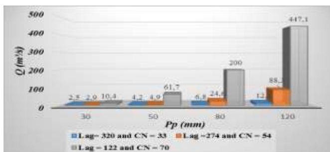
Fig. 6 Simulated flows in current conditions of afforestation for different amounts rainfall fallen in 3hour
