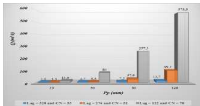
Fig. 5 Simulated flows in current conditions of afforestation for different amounts rainfall fallen in 1 hour
