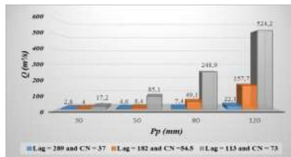
Fig. 12 Simulated flows in conditions of deforestation degree of 15% for different amounts rainfall fallen in 3 hour
