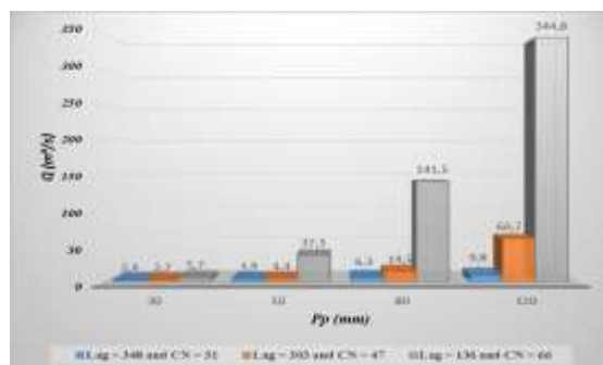
Fig. 9 Simulated flows in conditions of afforestation degree of 80% for different amounts rainfall fallen in 3hour
