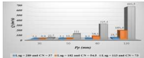
Fig. 11 Simulated flows in conditions of deforestation degree of 15% for different amounts rainfall fallen in 1 hour
