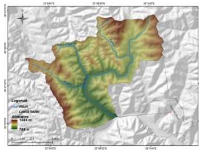
Fig. 1 Valea Rece basin location in Romania
